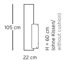
Armlehne (inkl. Armlehnenkissen) Armrest (with armrest cushion)
